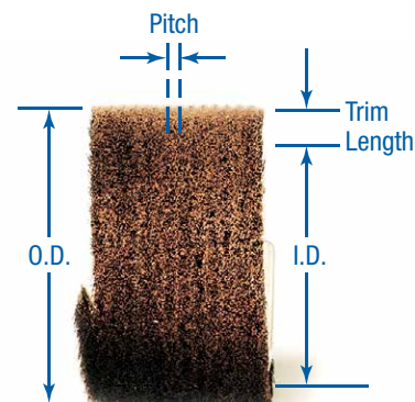
Close Wound Pitch for a full brush
